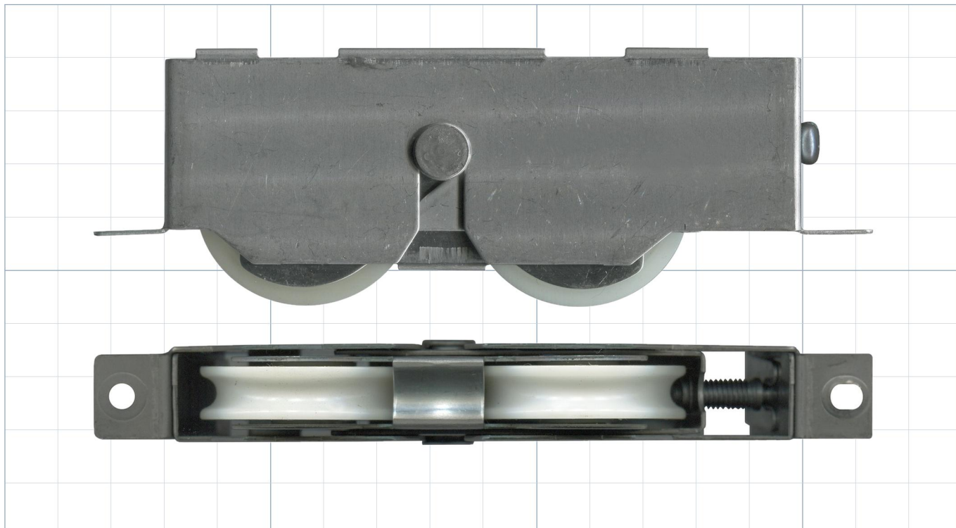
146.8mm Adjustable Sliding Door Carriage & Roller
