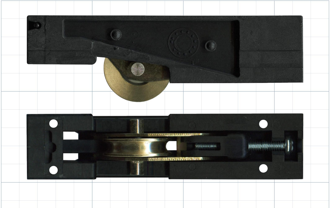
152.3mm Adjustable Sliding Door Carriage & Roller
