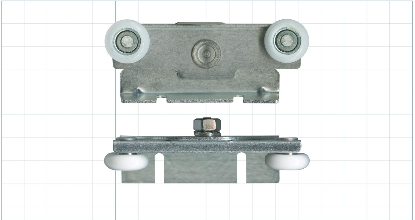
20mm Sliding Door Trolley & Nylon Roller – Wardrobe Top Hung Steel
