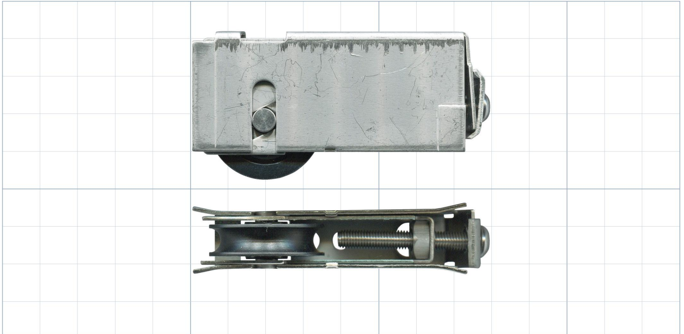
32mm Adjustable Sliding Door Carriage & Roller
