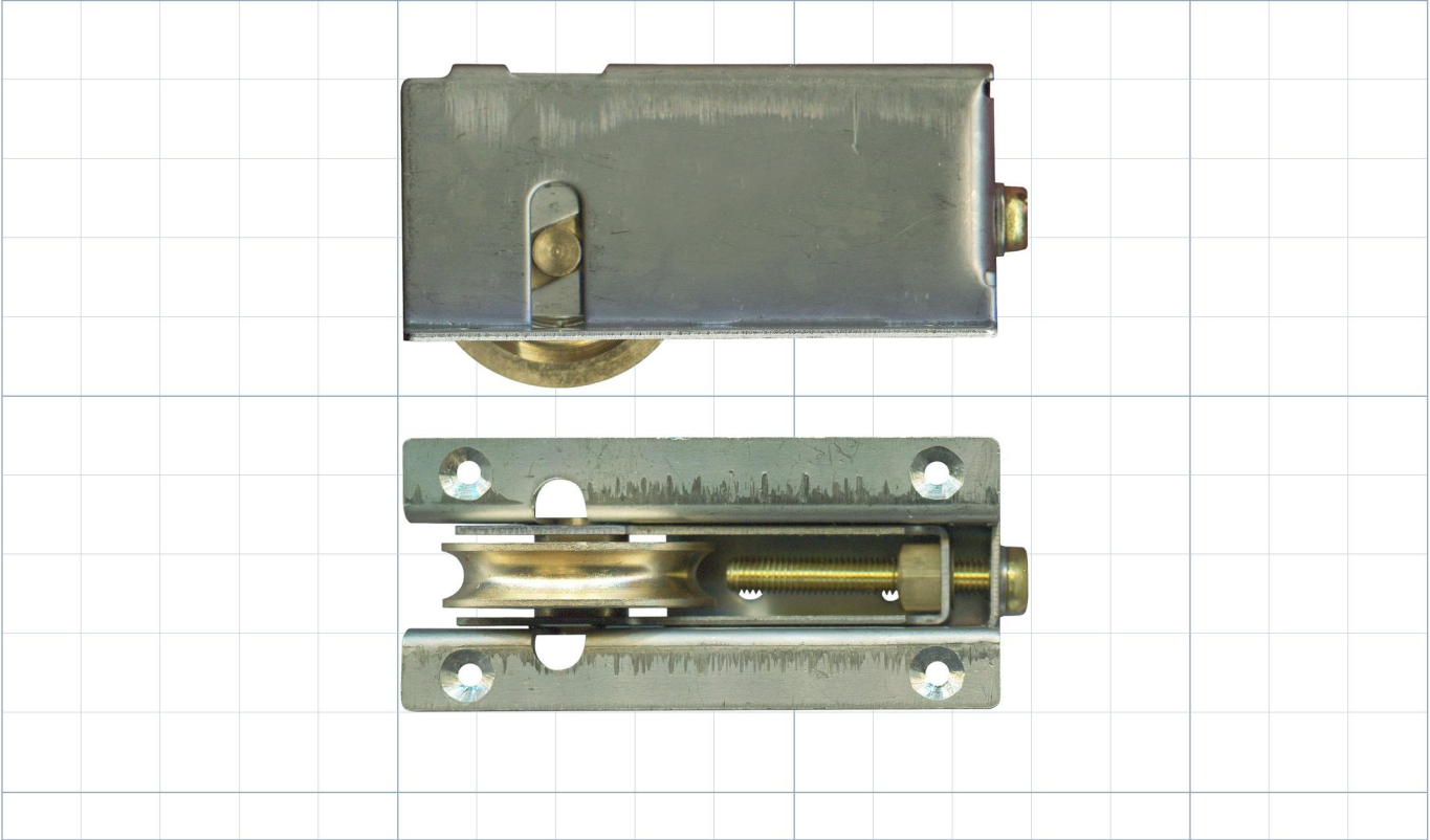
79.4mm Adjustable Sliding Door Carriage & Roller
