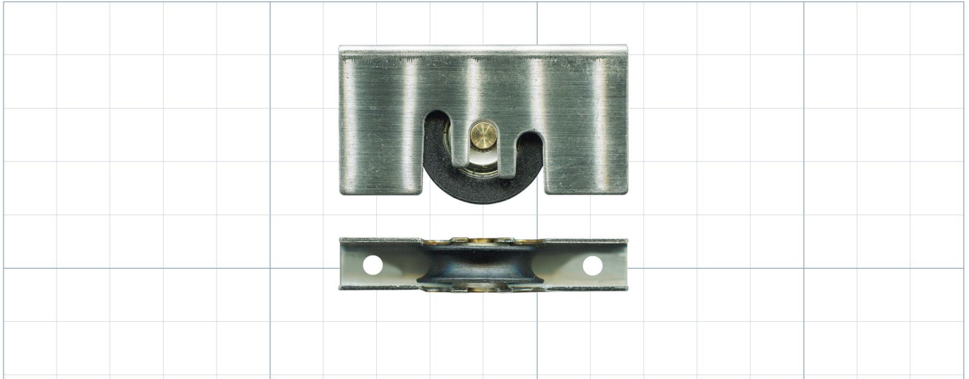
25kg Stainless Steel Adjustable Window Carriage & Roller
