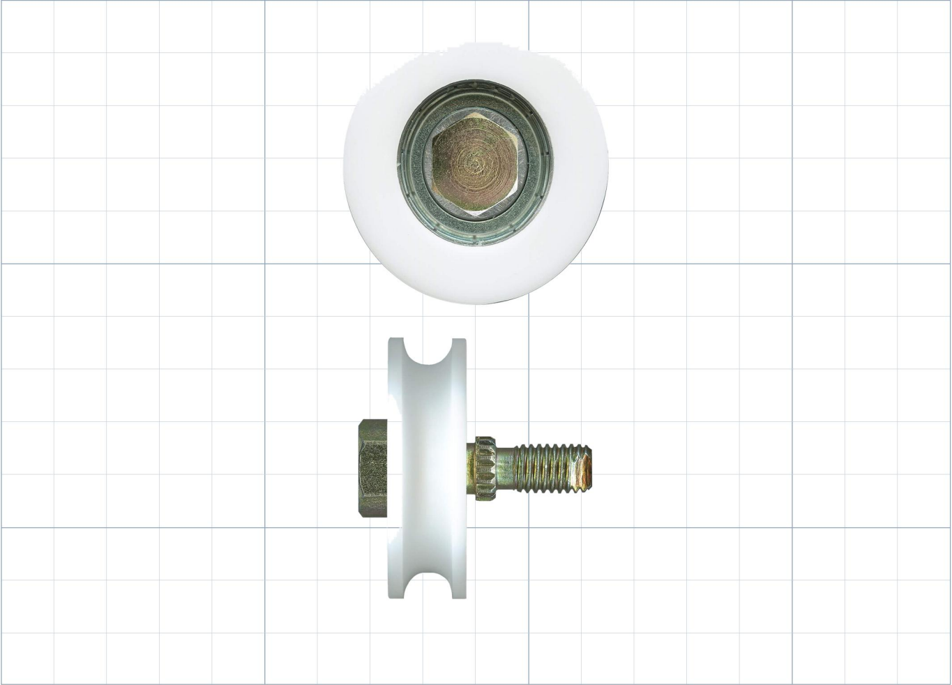
50.6mm Sliding Door Roller – Suits Commercial Hanging Doors
